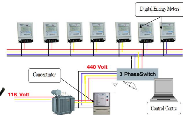
Figure 1: Detail Model of smart grid with EAWHR
